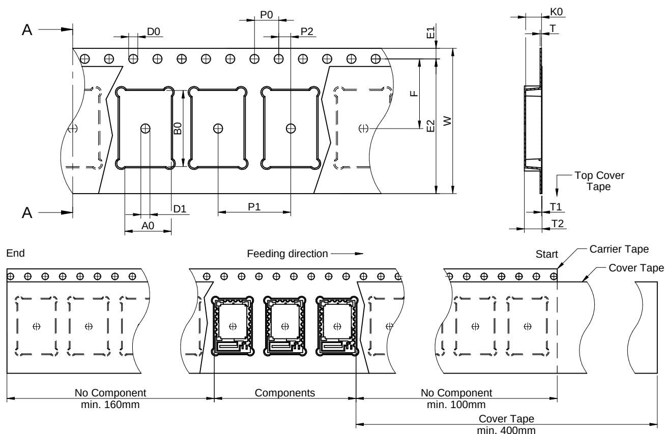
Figure 28: 24 mm Tape
