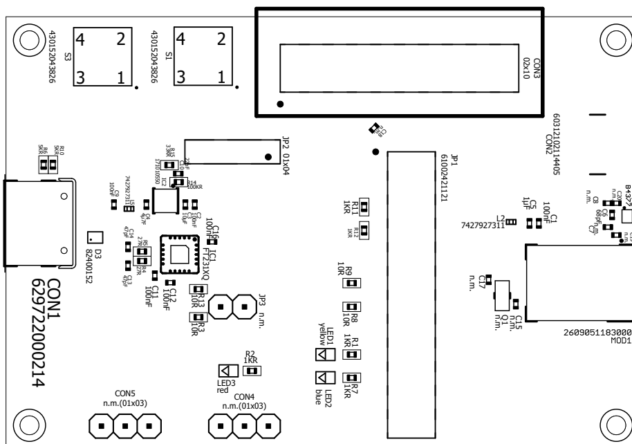
Figure 19: Assembly diagram
